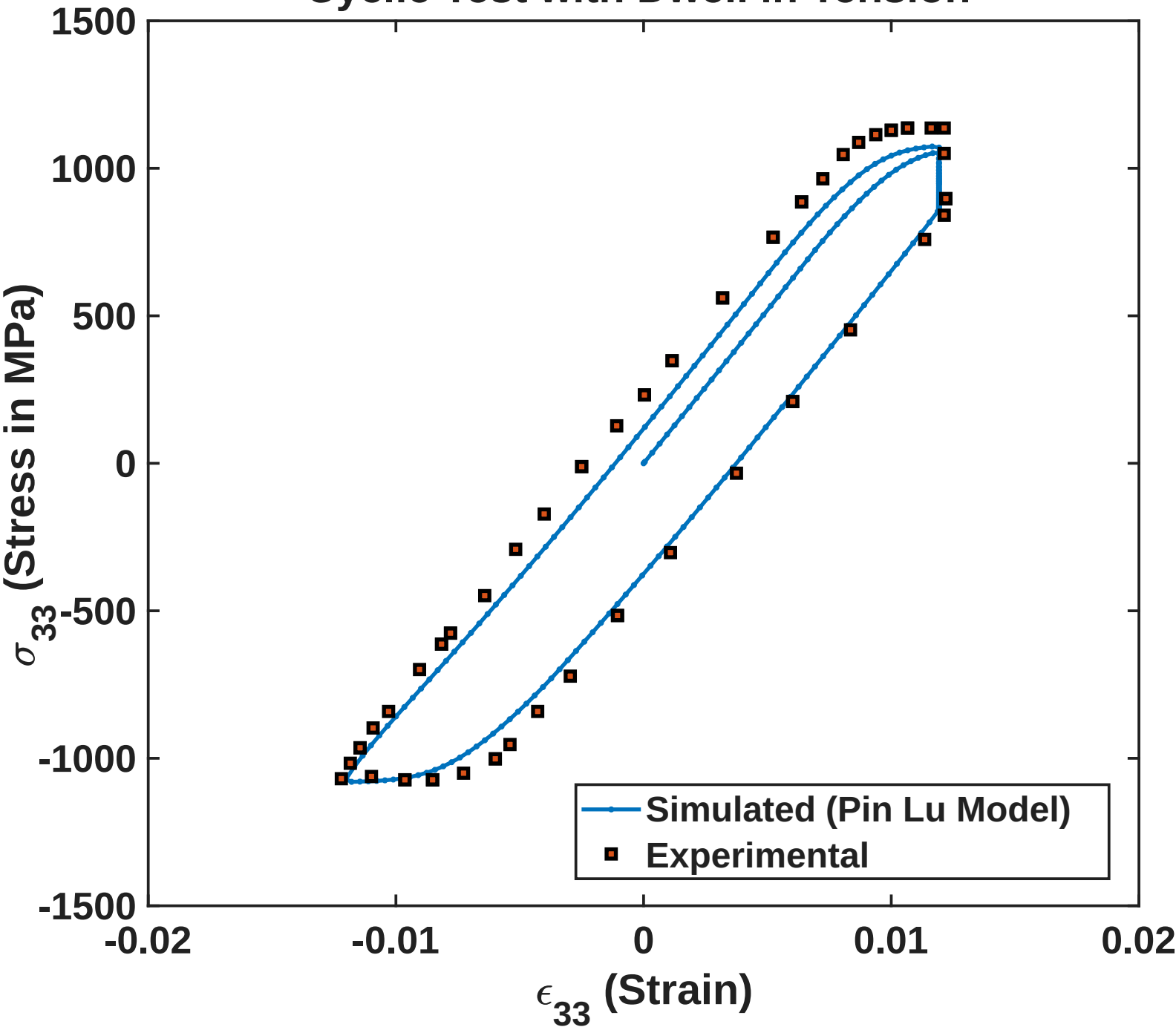
Cyclic Test with Dwell in Tension
